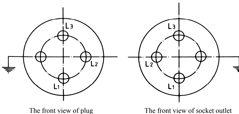
Fig. 22.4.4.3. Sequence of phase connections of plug and socket outlet
